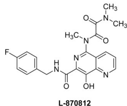
Fig. 1. The structure of L-870812, a naphthyridine carboxamide that inhibits the strand-transfer activity of recombinant HIV and SIV integrase in vitro (IC 50 = 40 nM).
